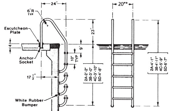
SRS-RLF-24S-xx Residential Ladder
