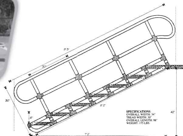
POOL LIFT SRS-200
