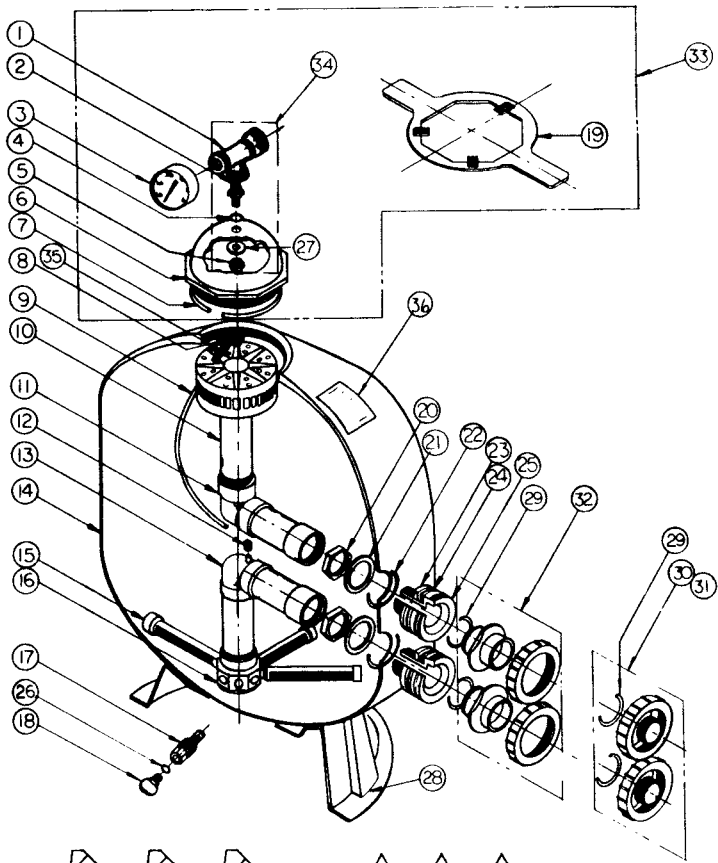
6" BUTTRESS THREAD
