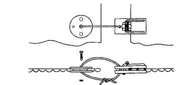
2304 Tandem connector kit (4)
