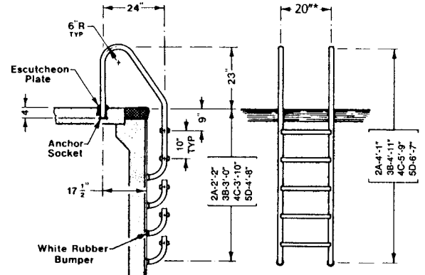
SRS-RLF-24S-xx Residential Ladder
